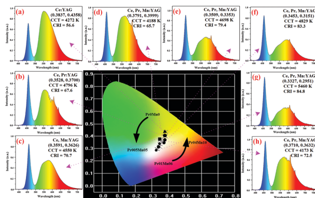
Fig. 6 Electroluminescence spectra and chromaticity parameters of the corresponding white LEDs driven by a 350 mA current: (a) \text{PrO Mn0} , (b) \text{PrO2 Mn0} , (c) \text{PrO Mn04} , (d–h) \text{PrO05 Mn05} , \text{PrO1 Mn06} , \text{PrO15 Mn07} , \text{PrO2 Mn08} , \text{PrO4 Mn10} .
