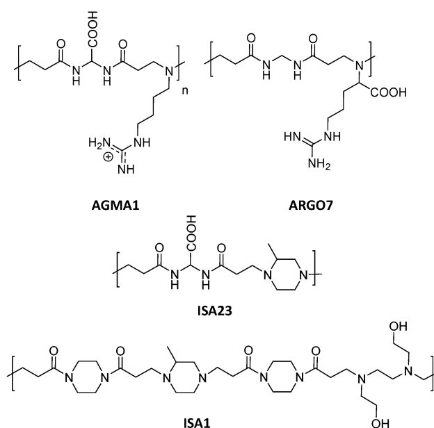
Fig. 5 Chemical structures of AGMA1, ISA23, ISA1 and ARGO7. 95,96
