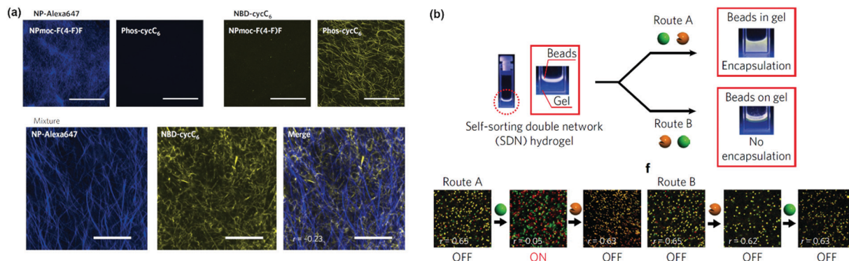
Fig. 8 (a) The visualisation of the self-sorting of redox-responsive NPmoc-F(4-F)F, labelled with an Alexa647 dye, and peptide amphiphile Phos-cycC 6 labelled with NBD (scale bar 50 μm). (b) Control of nanobead encapsulation through orthogonal stimuli, where the order of external stimulus application (sodium dithionite, green sphere or bacterial alkaline phosphatase, orange sphere) controls nanobead motion. 79 Copyright 2018, Nature Publishing Group.
