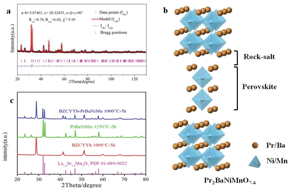
Fig. 2 (a) Rietveld refinement plot of PrBaNiMn powder using X-ray powder diffraction data, R_{wp} and \chi^2 represent the weighted profile factor and reduced chi-square; (b) the crystal structure of Pr 2 BaNiMnO 7.8 ; (c) XRD patterns of PrBaNiMn, BZCYYb fired at 1250, 1000 °C and the dry-mixed composite powder BZCYYb–PrBaNiMn (5 : 5) fired at 1000 °C for 5 h, respectively.
