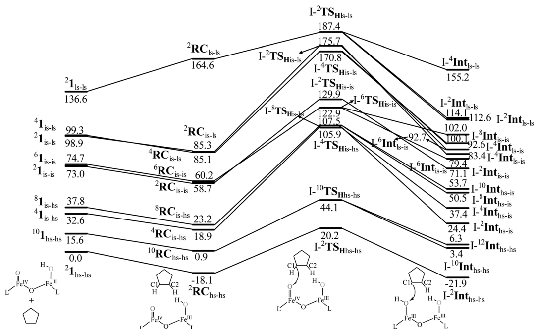
Fig. 2 B3LYP-D3 computed energy for the C–H bond hydroxylation of cyclopentane (CP) by species 1 (energies are in kJ mol -1 ).
