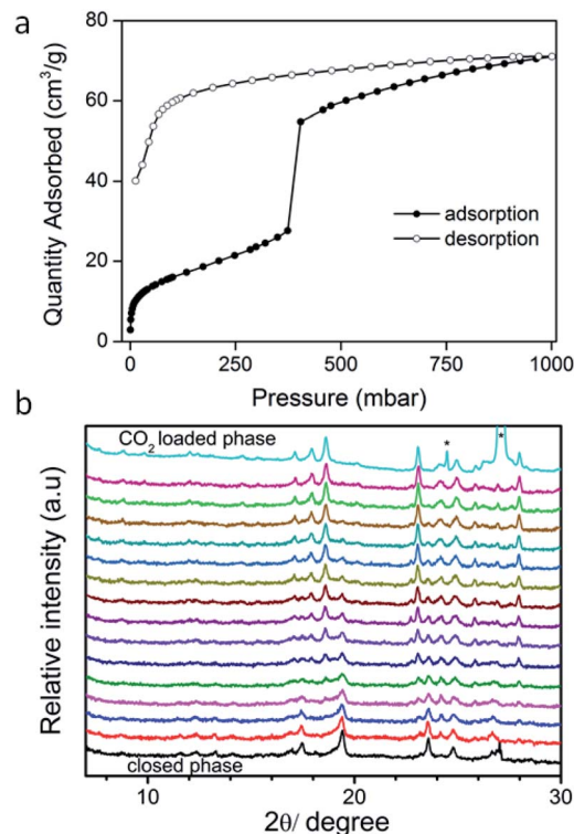
Fig. 3 Activated \text{sql-1,3-Co-NCS} (closed phase), (a) 195 K \text{CO}_2 isotherm; (b) time-dependent (data collection interval: 5 min, 25 min spent on collection of the top \text{CO}_2 loaded pattern) in situ PXRD patterns recorded upon dosing \text{CO}_2 (900 mbar) at 195 K. Peaks labelled * correspond to dry ice.
