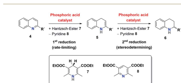
Scheme 3 Two-step transfer-hydrogenation of quinolines 4 to tetrahydroquinolines 6 .
