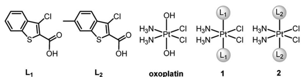
Fig. 1 Chemical structures of ligands L 1 and L 2 , oxoplatin and complexes 1 and 2 .
