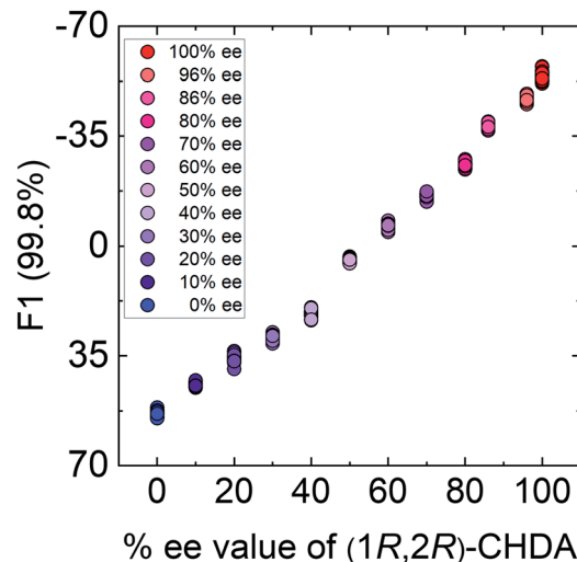
Fig. 8 Results of the semi-quantitative assay based on LDA for the determination of % ee in (1R,2R)-CHDA. Twenty repetitions were conducted for each % ee.
