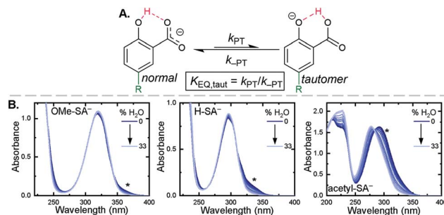
Fig. 2 (A) Salicylate proton-transfer tautomer. The normal and tautomeric forms are labelled. (B) Absorption spectral changes upon the addition of increasing amounts of H 2 O to CH 3 CN solutions of the indicated salicylate derivatives, ~250 μM. Asterisks mark the tautomer absorbance.
