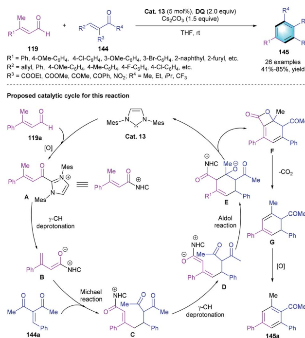
Scheme 42 NHC-catalyzed [3 + 3] benzannulation to synthesize polyfunctionalized benzenes.
