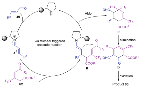
c) Synthesis of biaryls through RC-type reaction
