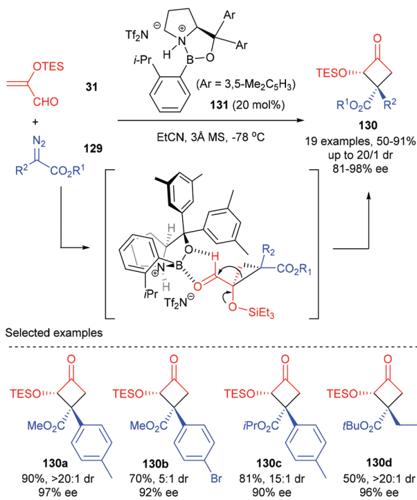
Scheme 37 Tandem cyclopropanation/semipinacol rearrangement.
