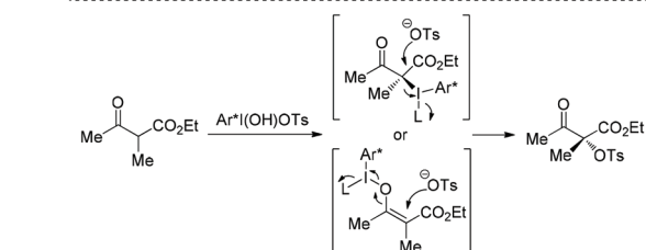
Scheme 52 Asymmetric oxidation of \alpha -substituted \beta -ketoesters promoted by C_2 -symmetric iodoarene.
