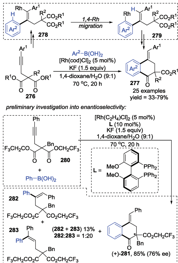
Scheme 47 Rh-Catalyzed arylytic cyclization of alkynyl malonates with arylboronic acids.
