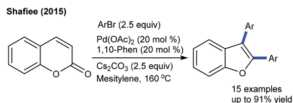
Scheme 11 Domino C–H and C–C activation of coumarins.
