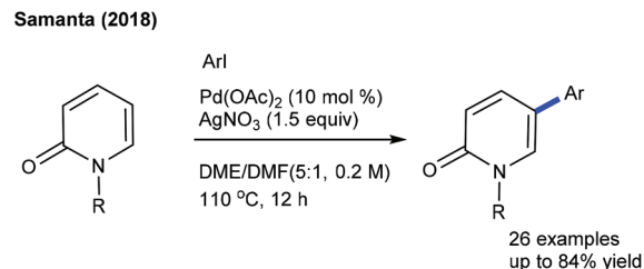
Scheme 9 C5-Arylation of pyridones.
