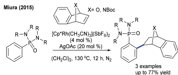
Scheme 64 Functionalization of arylphosphoramides.
