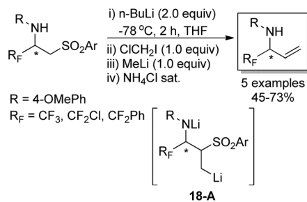
Scheme 18 Asymmetric synthesis of allylic amines.
