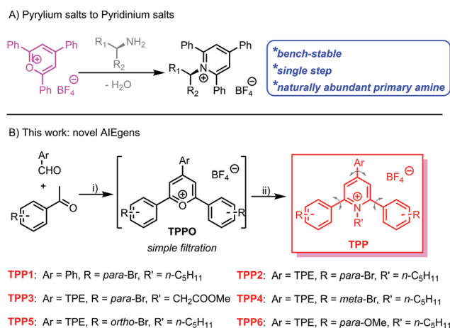
Scheme 1 (A) Facile synthesis of Katritzky pyridinium salts from the corresponding pyrylium precursors. (B) Synthetic routes toward novel AIEgens based on Katritzky salts. Conditions: (i) \text{BF}_3 \cdot \text{Et}_2\text{O} , toluene, 80 °C, 46% ( TPPO1 ), 45% ( TPPO2 ), 38% ( TPPO3 ), 19% ( TPPO4 ), 50% ( TPPO5 ); (ii) primary amine, ethanol, 80 °C, 69% ( TPP1 ), 92% ( TPP2 ), 86% ( TPP3 ), 83% ( TPP4 ), 66% ( TPP5 ), 98% ( TPP6 ).
