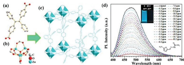
Fig. 3 (a) The BCTPE^{2-} ligand, (b) the Zn_4O(CO_2)_6 cluster in (c) the 3D structure. (d) Luminescence titration of this LMOF in aqueous solution at various NFZ concentrations. Inset: the optical photos at 0 and 65.5 ppm (NFZ). Reproduced from ref. 78 with permission from The Royal Society of Chemistry.
