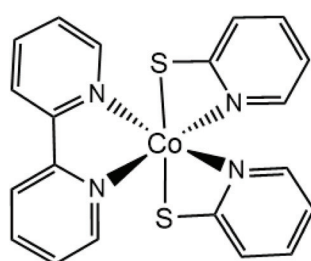
Scheme 18 Molecular structures of metal pyridine–thiolate HER catalysts.
