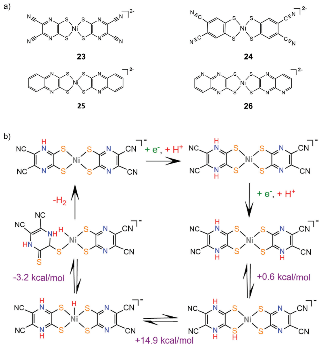
Scheme 14 (a) HER catalysts carrying substituent qdt ligands. (b) Proposed mechanism catalysed by complex 23 .
