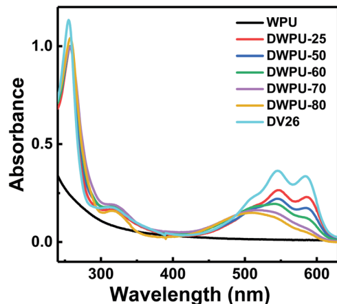
Fig. 1 The UV absorption spectra of DWPUs.
