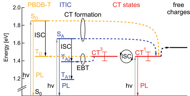
Fig. 5 Jablonski diagram of the PBDB-T:ITIC blend. S_D , T_D – singlet and triplet excited states of the donor PBDB-T (yellow). S_A , T_{A1} , T_{A2} – singlet and two triplet states of the acceptor ITIC (blue). CT^1 , CT^3 – singlet and triplet charge transfer states (red), ISC – intersystem crossing, EBT – electron back transfer.
