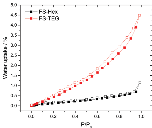
Fig. 3 Water vapor isotherms of FS-Hex and FS-TEG at 20.0 \text{ °C} and up to 23 \text{ mbar} .
