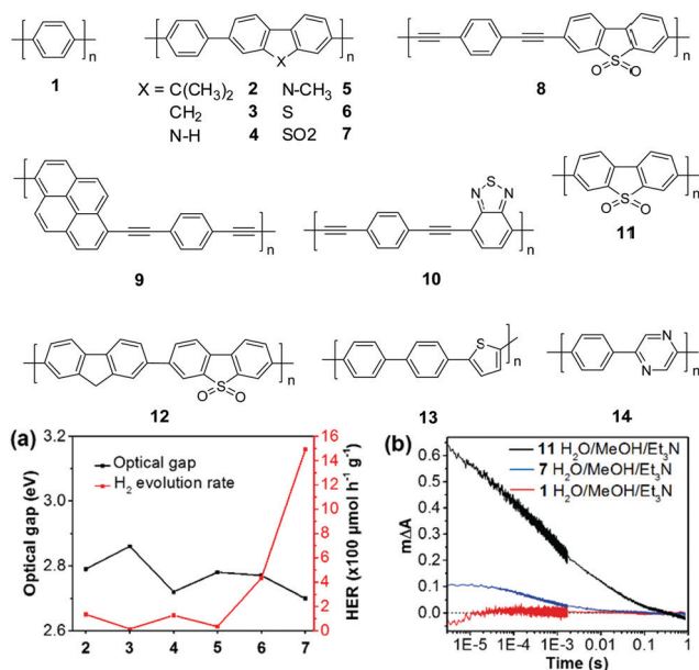
Fig. 5 Chemical structures of polymers 1–14, (a) the correlation between the photocatalytic \text{H}_2 evolution and their optical gaps of polymers 2–7 ( >420 \text{ nm} ); (b) transient kinetics probed at 630 \text{ nm} for polymers 1, 7, and 11 in the \text{Et}_3\text{N}/\text{CH}_3\text{OH}/\text{H}_2\text{O} mixture (excited at 355 \text{ nm} ). Reprinted with permission from ref. 72. Copyright 2018 Nature Publishing Group.
