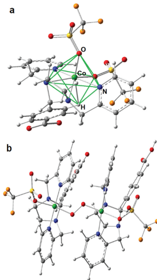
Fig. 3 (a) The DFT calculated coordination environment of the individual Co-centers in Co 4 L1 , which matches best with the experimental data. The straight green lines reveal the N-capped \text{O}_2\text{N}_3\text{H} -octahedron environment of the central Co(II) center, by taking into account the agostic C–H...Co interaction. (b) DFT model of 1 with fixed carboxylate C...C atom distance of 6.43123 Å according to the XRD structure of the free ligand. In 1 , L1 acts as a tetradentate ligand with one of the nitrogen atoms staying away from the coordination environment of Co.
