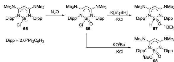
Scheme 25 Activation of N_2O by the chlorosilylene 65 and further metathesis reaction at the Si centre.
