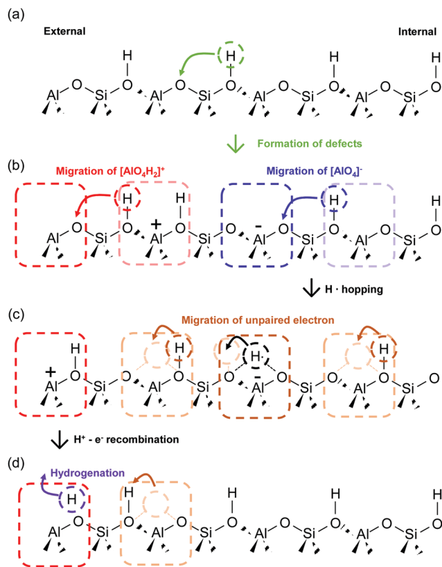
Fig. 10 Schematic images of H atoms migration mechanism over aluminosilicate. (a) Generation of [AlO_4H_2]^+ and [AlO_4]^- by H^+ migration. (b) Subsequent H atoms migration at both [AlO_4H_2]^+ and [AlO_4]^- . As for the migration at [AlO_4]^- , [AlO_4]^- H^* is formed. (c) Migration of unpaired electron. H^+ reached to the external support surface recombines with the electron. (d) Hydrogenation of hydrocarbons using H^+ at the external support.
