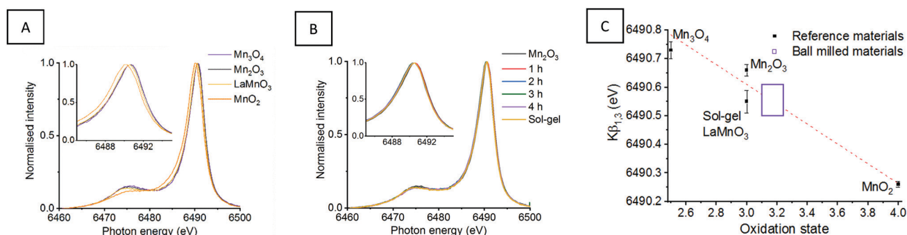
Fig. 2 Mn K \beta XES mainlines for (A) Mn reference oxides and sol-gel synthesised LaMnO 3 with (B) 'time-slices' during the mechanochemical synthesis of LaMnO 3 (C) presents the K \beta 1,3 max as a function of oxidation state, with a line of best fit calculated from the reference materials and used to calculate the oxidation state of the ball milled materials. 11
