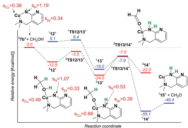
Fig. 5 Potential energy surface for the reaction of ^37b^+ with methanol calculated at the B3LYP level with the 6-311+G(2d,p) basis set for copper and 6-31+G* basis set for all other atoms. The relative energies refer to 0 K and are in kcal mol -1 . The spin densities were obtained from Mulliken analysis at the B3LYP/6-311G(2d,p) level. The structures are displayed with a truncated ligand, but all the calculations were performed with the full ligand.
