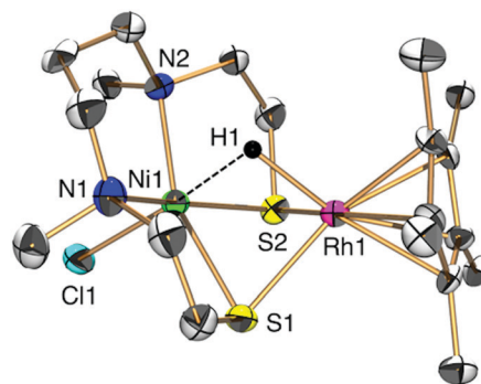
Fig. 1 ORTEP drawing of 2 with ellipsoids set at the 50% probability level. The hydrogen atoms of the ligand X ( N,N' -dimethyl-3,7-diazanonane-1,9-dithiolato) and C 5 Me 5 are omitted for clarity. Selected interatomic distances [Å] and angles [°]: Ni1···Rh1 2.7454(16), Rh1–H1 1.84(9), Ni1–H1 1.96(9), Ni1–S1–Rh1 71.15(7) and Ni1–S2–Rh1 70.65(7) for 2 .
