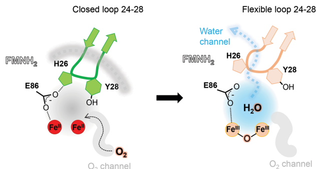
Fig. 3 Contribution of the hydrophobic O_2 -channel, loop 24–28 and water channel in the catalytic mechanism. The hydrophobic O_2 -channel (gray) and hydrophilic water-channels (light blue) are indicated. In the reduced state, the loop is closed and fixed (green and gray dashed line). After the first water is produced, the switch loop is still closed but becomes flexible (orange), where the water is released to bulk solvent.
