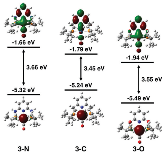
Fig. 3 DFT calculated HOMO and LUMO energy levels of 3-N (left), 3-C (middle), and 3-O (right). 3-N has the highest LUMO despite having a lower HOMO energy than 3-C . This high-energy LUMO is correlated with the more negative reduction potential of 3-N .
