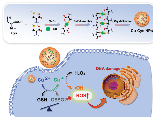
Fig. 12 Schematic illustration of the synthesis, modification, and proposed mechanism of Cu–Cys NPs for enhanced CDT. Reprinted with permission from ref. 43. Copyright (2019) American Chemical Society.
