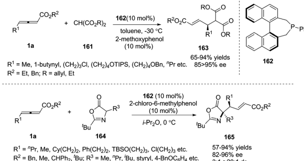
Scheme 51 Phosphine-catalyzed asymmetric additions of \gamma -substituted allenates and carbon electrophiles.
