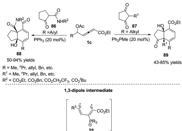
Scheme 28 Phosphine-catalyzed (4+2) annulations of \delta -acetoxy allenates and ketones.
