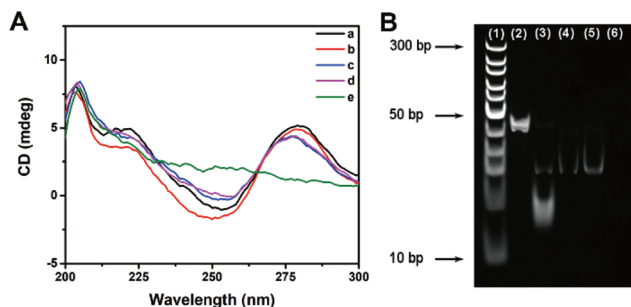
Fig. 2 (A) CD spectra of (a) dsDNA-1, (b) dsDNA-1 and Fpg, (c) dsDNA-1, Fpg and λ Exo, (d) dsDNA-1, Fpg, λ Exo and Exo I, and (e) dsDNA-1, λ Exo and Exo I. (B) PAGE image of different samples. Lane (1): DNA ladder, lane (2): dsDNA-1, lane (3): dsDNA-1 and Fpg, lane (4): dsDNA-1, Fpg and λ Exo, lane (5): dsDNA-1, Fpg, λ Exo and Exo I, and lane (6): dsDNA-1, λ Exo and Exo I.
