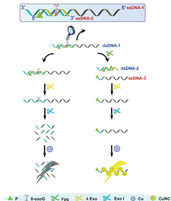
Fig. 1 Illustration of Fpg detection based on the distinct effects of P on λ Exo and Exo I along with CuNCs.
