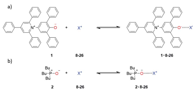
Scheme 2 Formation of H-bonded complexes between HBAs and cations.
