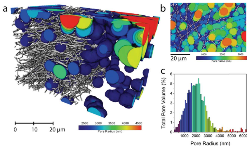
Fig. 2 Pore size distribution in the pore phase of the carbonized N0 sample. For clarity, the smaller pores have been removed in (a) and a 2D representation of all the calculated pore radii is shown in (b). The sphere radius was dilated by 100 nm at a time and the histogram of total pore volumes of each sphere radius is shown in (c).
