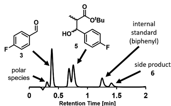
Fig. 4 Representative UPLC chromatogram showing all measured reaction components. The signal labelled “polar species” is comprised mostly of 4-fluorobenzoic acid, present as a minor impurity in aldehyde 3 .
