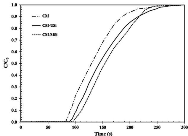
Fig. 8 Breakthrough curves of the NR latex foam, and the rubber composite of the CM foam filled with either USi (CM-USi) or MSi (CM-MSi) particles at a mixed gas flow rate of 100 mL min -1 under ambient temperature and pressure.
