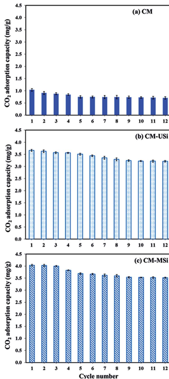
Fig. 9 The CO 2 uptake of (a) CM, (b) CM-USi and (c) CM-MSi foams over 12 adsorption–desorption cycles; adsorption: a mixed gas flow rate of 100 mL min -1 under ambient temperature and pressure; desorption: 60 °C under vacuum for 20 min.
