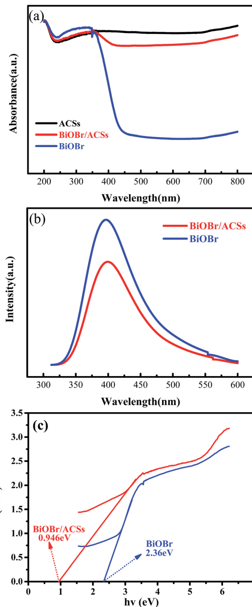
Fig. 4 (a) DRS of the as-prepared samples; (b) PL spectra of BiOBr and BiOBr/ACSSs samples; and (c) plots of (\alpha h\nu)^{1/2} versus photon energy ( h\nu ).
