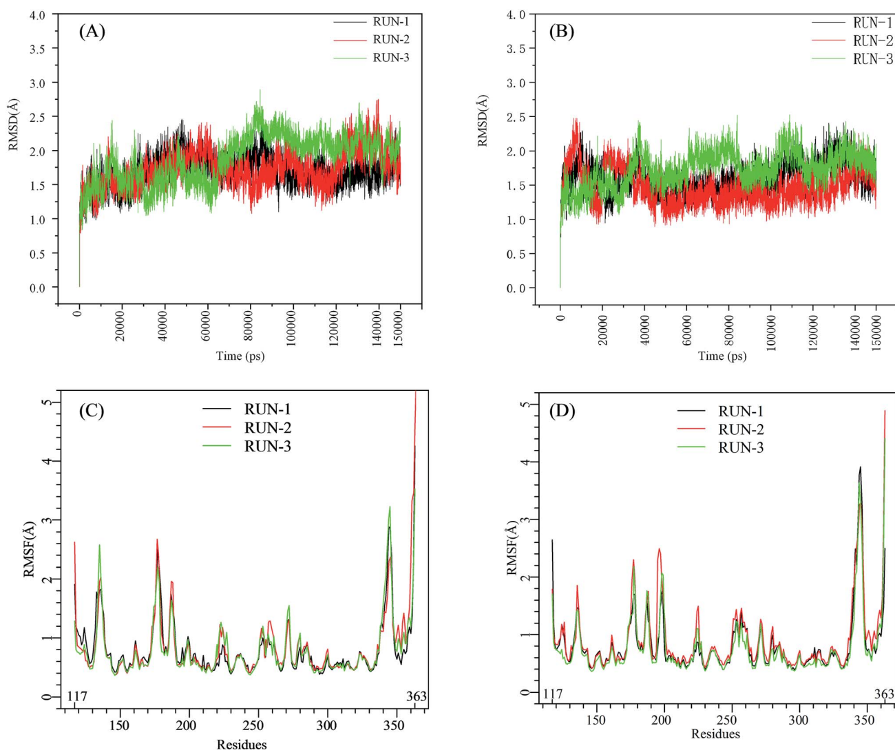
Fig. 1 RMSD and RMSF plots for ( R/S )-PFI-2/SETD7/SAM systems. Black, red, green: trajectories of three independent MD simulations (run-1, run-2, run-3). (A) and (B) are the RMSD plots of ( R )-PFI-2/SETD7/SAM system and ( S )-PFI-2/SETD7/SAM system, respectively. (C) and (D) are the RMSF plots of ( R )-PFI-2/SETD7/SAM system and ( S )-PFI-2/SETD7/SAM system, respectively.
