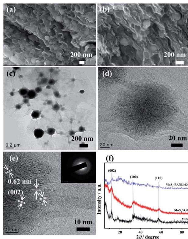
Fig. 2 (a) and (b) FE-SEM images of \text{MoS}_2 -PANI/rGO nanocomposite; (c) TEM and (d and e) HR-TEM images of 3D \text{MoS}_2 -PANI/rGO nanocomposite (the inset in (e) is the corresponding SAED pattern), and (f) XRD patterns of the \text{MoS}_2 , \text{MoS}_2 /rGO and \text{MoS}_2 -PANI/rGO samples.
