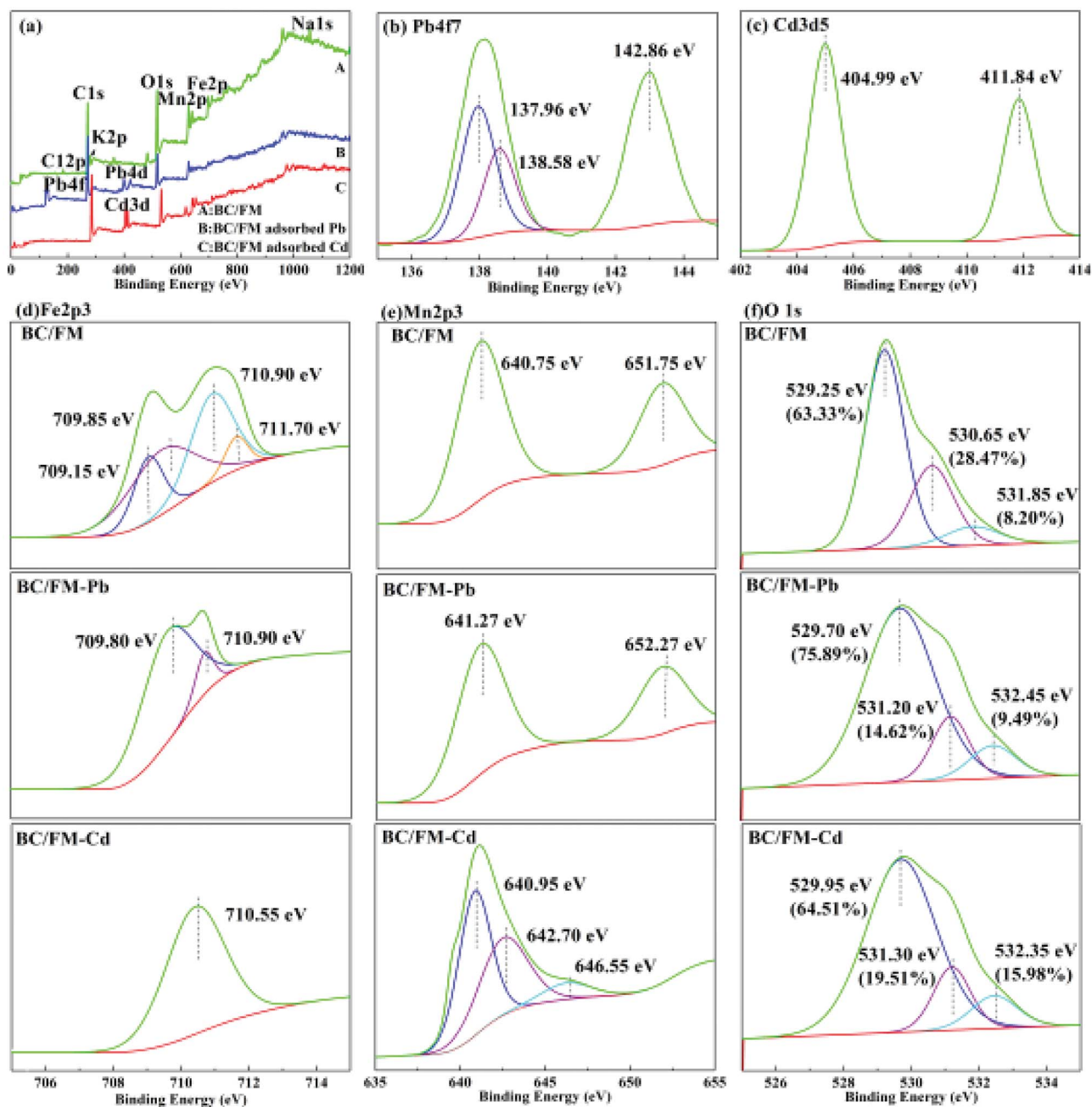
Fig. 10 XPS spectra of BC/FM before and after adsorption for \text{Pb(II)} and \text{Cd(II)} . (a) XPS spectra of BC/FM before and after \text{Pb(II)} and \text{Cd(II)} adsorption; (b) \text{Pb}4\text{f} XPS spectra of BC/FM-Pb; (c) \text{Cd}3\text{d} XPS spectra of BC/FM-Cd; (d) \text{Fe}2\text{p} XPS spectra of BC/FM, BC/FM-Pb and BC/FM-Cd; (e) \text{Mn}2\text{p} XPS spectra of BC/FM, BC/FM-Pb and BC/FM-Cd; (f) \text{O}1\text{s} XPS spectra of BC/FM, BC/FM-Pb and BC/FM-Cd.
