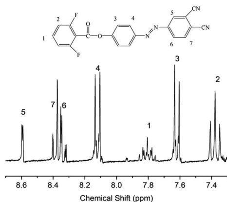
Fig. 2 1 H NMR spectrum of monomer 2 in DMSO-d 6 .
