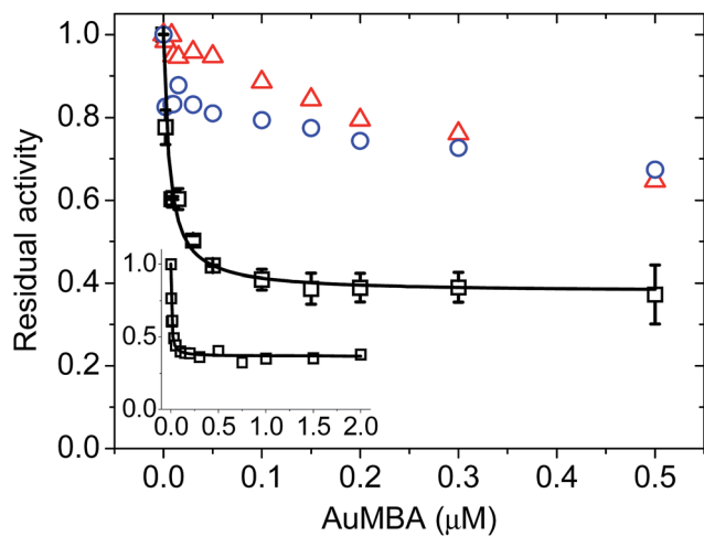
Fig. 7 Concentration-dependent inhibition of thrombin by AuMBA. Data obtained in the absence of competing ligands (squares) and in the presence of excess HD1 + HD22 (circles) and hirudin + HD22 (triangles). The inset shows the dose-response profile up to an AuMBA concentration of 2 \mu\text{M} . Thrombin concentration, 2 nM; HD1 and hirudin, 15 \mu\text{M} ; HD22, 5 \mu\text{M} ; S-2238, 100 \mu\text{M} . Assay performed in Tris-HCl buffer solution supplemented with 100 mM NaCl. Lines are a guide to the eye.
