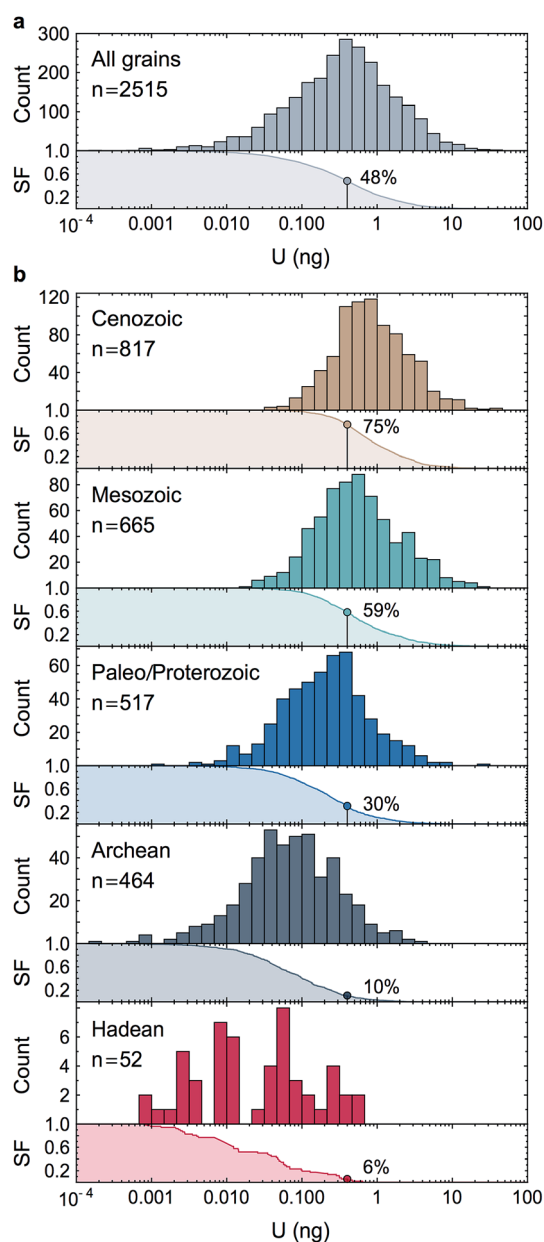
Fig. 7 Histograms and associated survival functions of post chemical abrasion U mass (in ng) recovered from 2515 individual zircon crystals analyzed in recent high-precision geochronology studies (data from ref. 23, 24, 35, 66, 67 and 70–94). (a) All data, (b), data shown by geological time periods. For each panel, the % of grains with more than 0.4 ng of U is shown on the survival function. The decrease in U content with increasing age is an artifact due to the chemical abrasion treatment. Indeed, radiation damages on the crystal lattice are more extensive in older zircons, resulting in greater proportion of the grain being leached away during the chemical abrasion step.
