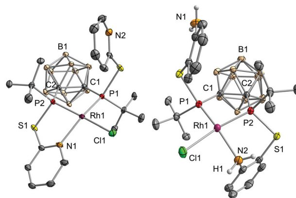
Fig. 2 Molecular structures of ( R_P, R_P )- 1 (left) and ( S_P, S_P )- 2 (right) in the solid state with ellipsoids drawn at the 50% probability level. All hydrogen atoms, except for those at the nitrogen atoms in 2 , are omitted for clarity. Selected bond lengths [Å] and angles [°]: 1 : Rh1–P1: 2.2028(6), Rh1–P2: 2.1417(6), Rh1–N1: 2.160(2), Rh1–Cl1: 2.3930(6), C1–C2: 1.702(3), P1–Rh1–P2: 90.77(2), P1–Rh1–N1: 156.06(5), P1–Rh1–Cl1: 99.45(2), P2–Rh1–N2: 84.43(6), P2–Rh1–Cl1: 165.09(2). 2 : Rh1–P1: 2.1958(8), Rh1–P2: 2.1605(9), Rh1–N2: 2.155(3), Rh1–Cl1: 2.396(1), C1–C2: 1.701(4), P1–Rh1–P2: 91.20(3), P1–Rh1–N2: 160.48(8), P1–Rh1–Cl1: 101.68(3), P2–Rh1–N2: 88.09(8), P2–Rh1–Cl1: 166.21(3).
