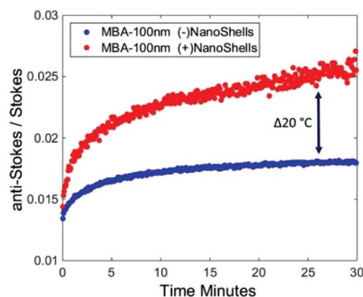
Fig. 3 Anti-Stokes/Stokes ratio of (1085 \text{cm}^{-1} 12 benzene ring mode) temperature reporter Au-MBA nanoparticles in the absence (blue) and presence (red) of Au-NS with a peak absorbance at 800 nm while inserted in porcine tissue at a depth of 5 mm (with a total thickness of 10 mm) and illuminated with 1.2 W ( \lambda_{\text{ex}} 830 nm). See ESI Fig. 2A & B† for corresponding raw Raman data.
