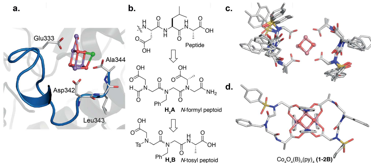
Fig. 2 (a) Selected amino acid residues from the D1 subunit (blue) that bind to the \text{Mn}_4\text{Ca} oxygen-evolving complex (OEC). (b) Design of the peptide analogues based on D1. (c) Ensemble of the five lowest energy NMR structures of 1-2B (pyridine ligands omitted for clarity). (d) The lowest energy structure of 1-2B .
