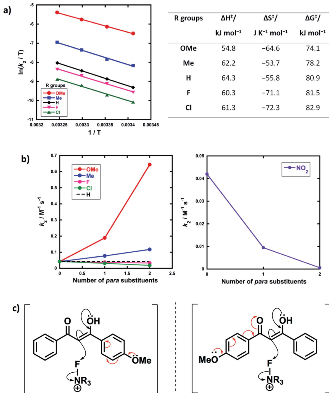
Fig. 6 (a) Eyring plots for fluorination of 1,3-dicarbonyls 1a–e by Selectfluor™ 3 in \text{CH}_3\text{CN} at 20 °C, 25 °C, 30 °C and 35 °C, and associated activation parameters. (b) Effect of mono- vs. di-substitution on the rate of fluorination; all rate constants were obtained in \text{CH}_3\text{CN} at 25 °C. (c) Asymmetry of the enol in the transition state.
