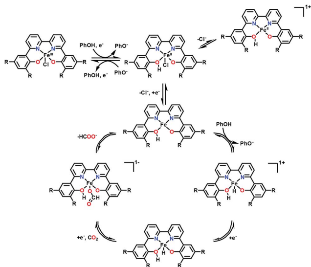
Scheme 8 Catalytic cycle for two-electron reduction of CO 2 to CO with a nonheme iron(III) chloride bearing a 6,6'-di(3,5-di- tert -butyl-2-hydroxybenzene)-2,2'-bipyridine ligand (Fe (tbu) dhbpy)Cl) via protonation by phenol. Reprinted with permission from ref. 127. Copyright 2018, American Chemical Society.
